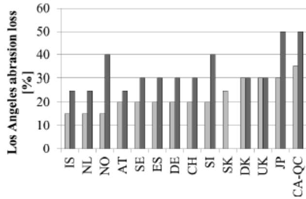
Figure 8. Upper limits for Los Angeles abrasion loss for aggregates used in bitumen bound materials.
