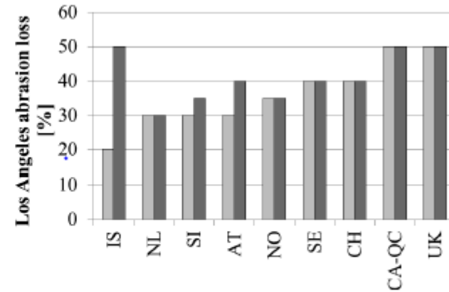
Figure 10. Upper limits for Los Angeles abrasion loss for unbound materials.
